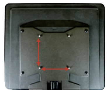
VESA Mount 75*75 mm
